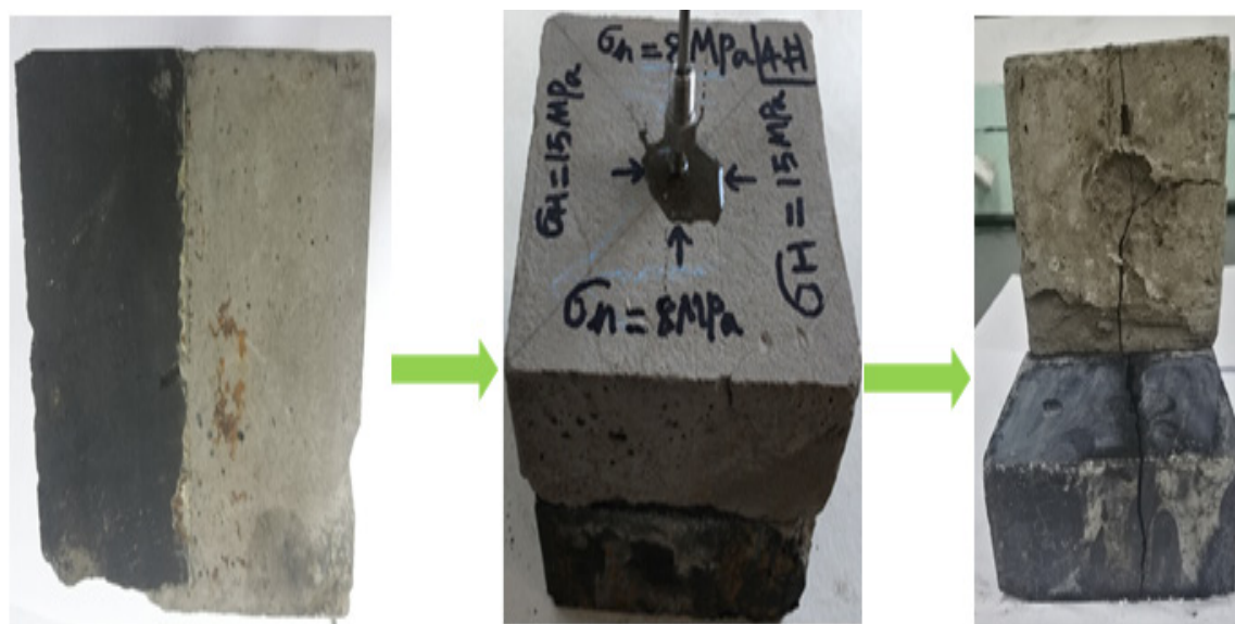
Figure 1. A fracture pattern of indirect fracturing of 100×100×100 mm specimen combination (top: sandy mud stone, bottom: coal)
