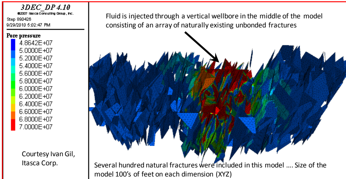
Figure 10: Three-Dimensional DEM Simulation of Hydraulic Injection into a Fractured Medium
