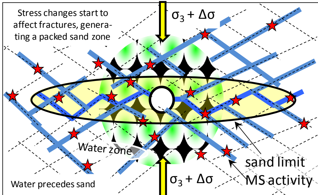
Figure 6: Water Travels Farther than Sand (filtration [6], bridging, settlement, hindered motion of aggregates), Stresses Change, + MS Activity...
