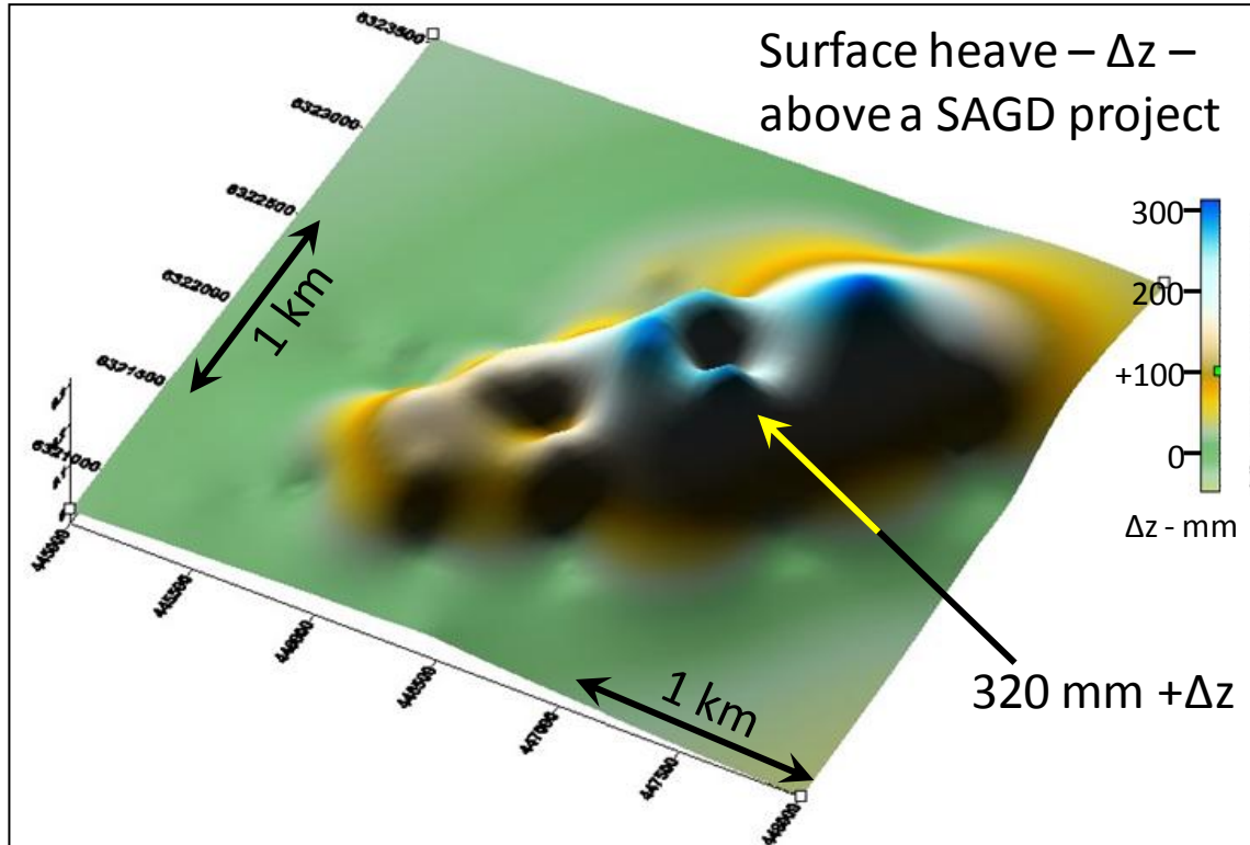
Figure 9: Surface Uplift above a Steam Injection Project
