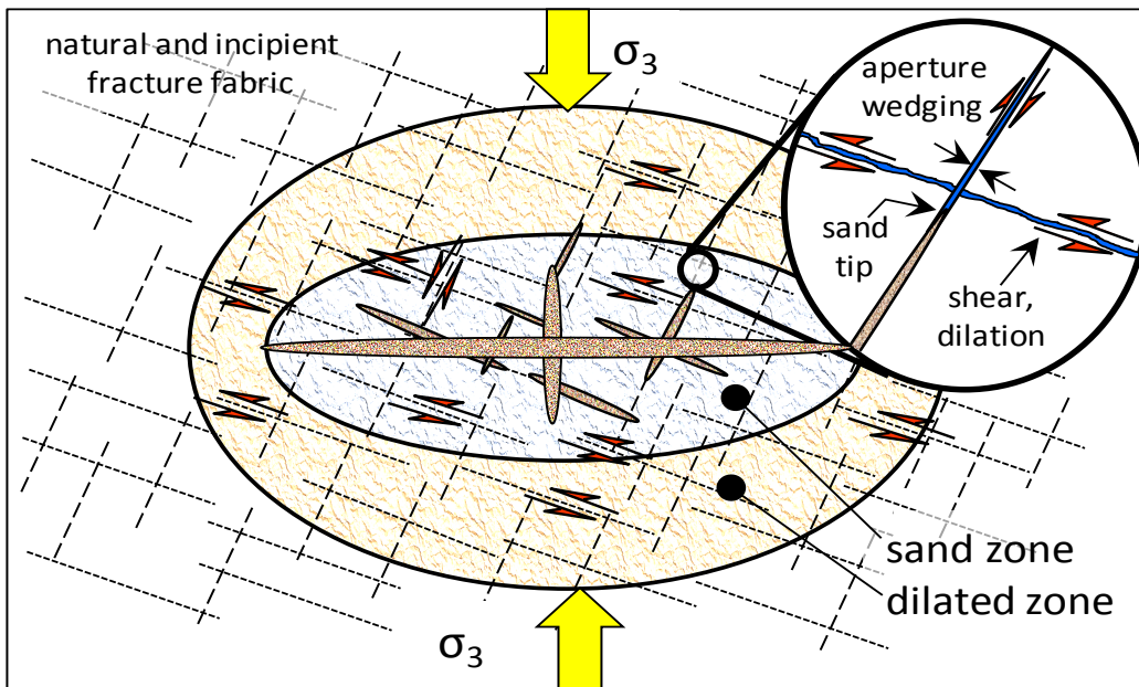
Figure 2: Plan View of the Sand Zone and the Dilated Zone around an MMHF Stage
