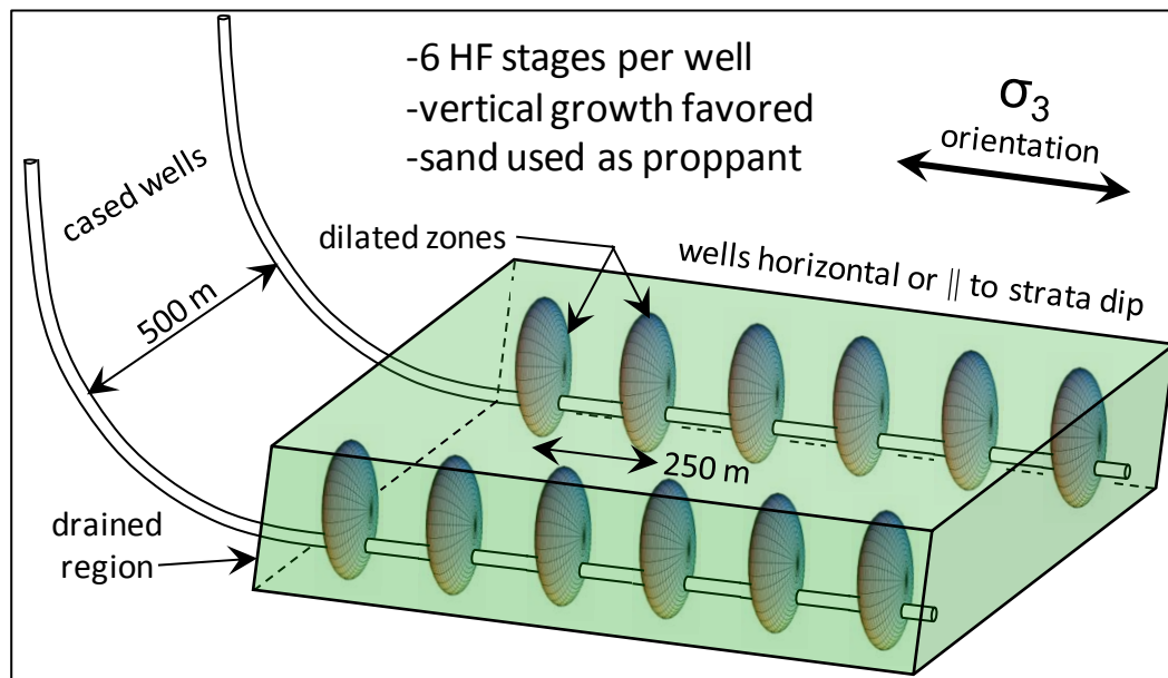
Figure 1: Multiple HF Stages along the Well Axis for Shale Gas Stimulation
