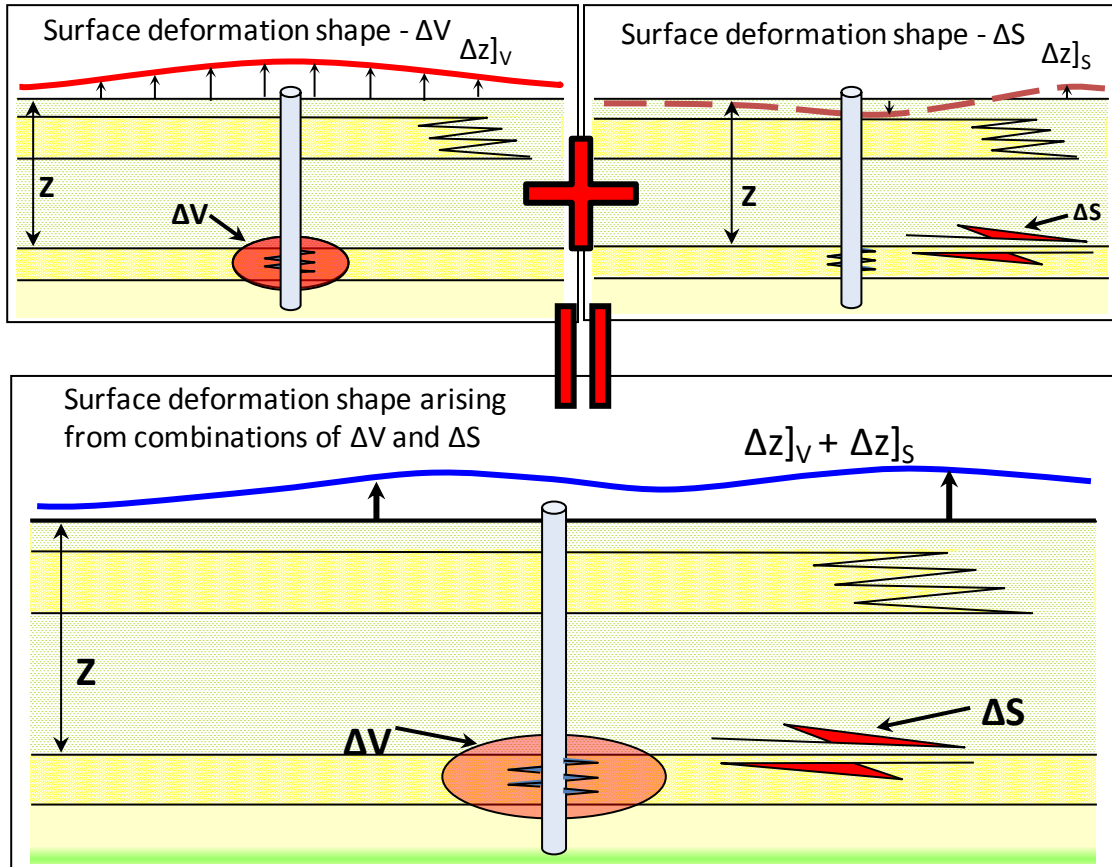
Figure 8: Surface Deformation Decomposition
