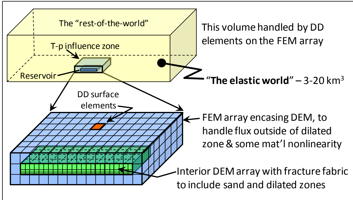
Figure 11: Embedded DEM in a FEM Array Coated with DD Elements to Simulate “the World”
