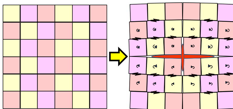
Figure 5: Rotations of Rigid Blocks (propping, wedging, rotation and shear can all be seen in the distorted array of blocks)
